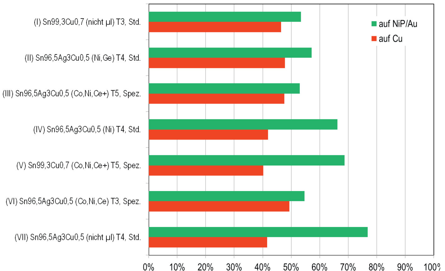
Fig. 8: Standardised shear forces after 1000 temperature cycles
