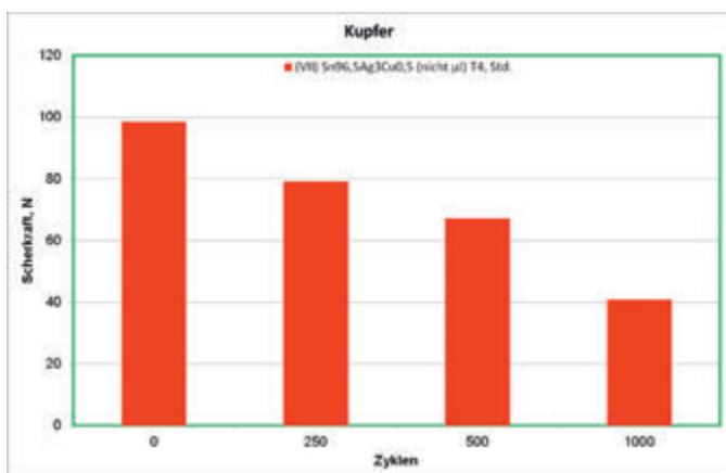
Fig. 1: Shear strength of 1206 chip resistors on Cu or NiP/Au PCB after 0, 250, 500, 1000 temperature cycles -25/+150 °C, soldered with VII AP-20 Sn96.5Ag3.0Cu0.5 T4, non-microalloyed
