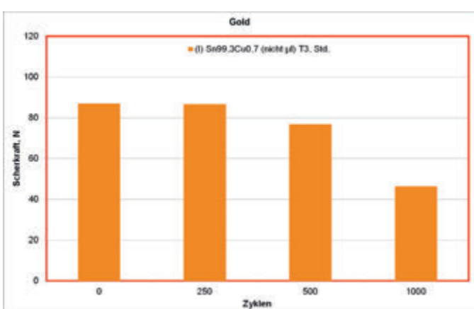
Fig. 2: Shear strength of 1206 chip resistors on Cu or NiP/Au PCB after 0, 250, 500, 1000 temperature cycles -25/+150 °C, soldered with I AP-20 Sn99.3Cu0.7 T3, non-microalloyed
