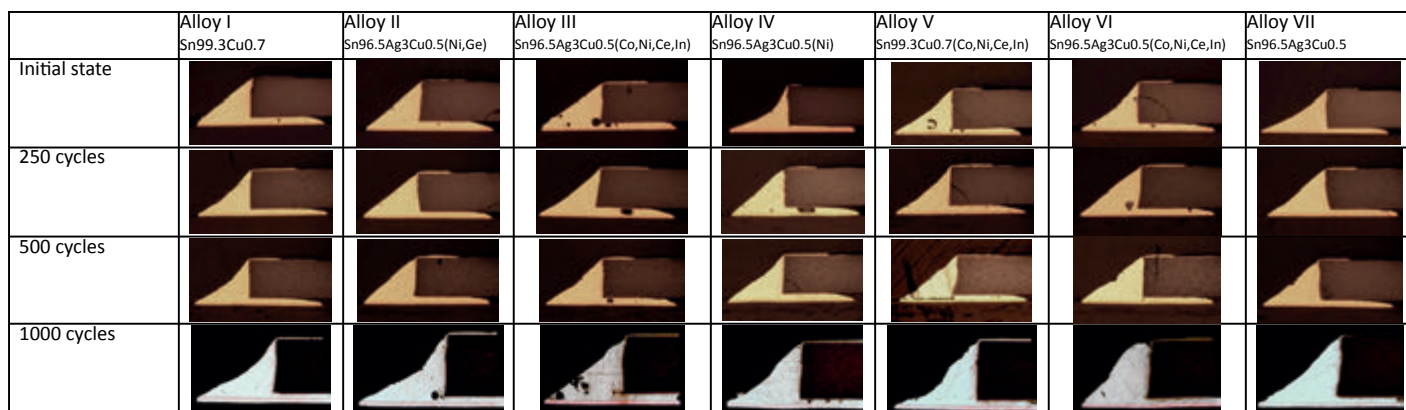
Fig. 6: Microsections on NiP/Au PCB
