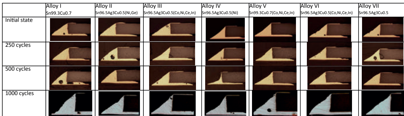
Fig. 5: Microsections on Cu PCB
